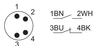
Fig. 7 1 NO + 1 NC (without LED)
