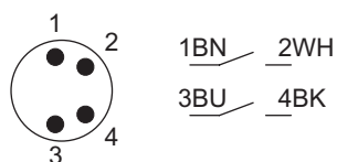
Fig. 5 2 NO (without LED)
